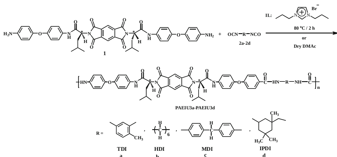
Scheme 1 Polymerization reactions of monomer 1 with several aromatic and aliphatic diisocyanates in IL or organic solvent
