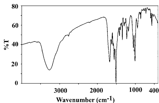
Fig. 1 FT-IR spectrum of PAEIU3c as a typical example
