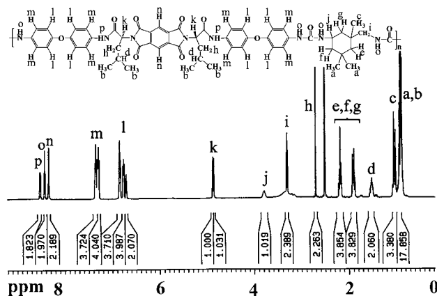
Fig. 2 1 H-NMR spectrum of PAEIU3d
